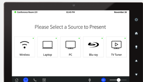
User Interfaces
